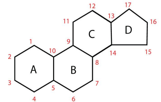
(a) Steroid skeleton
